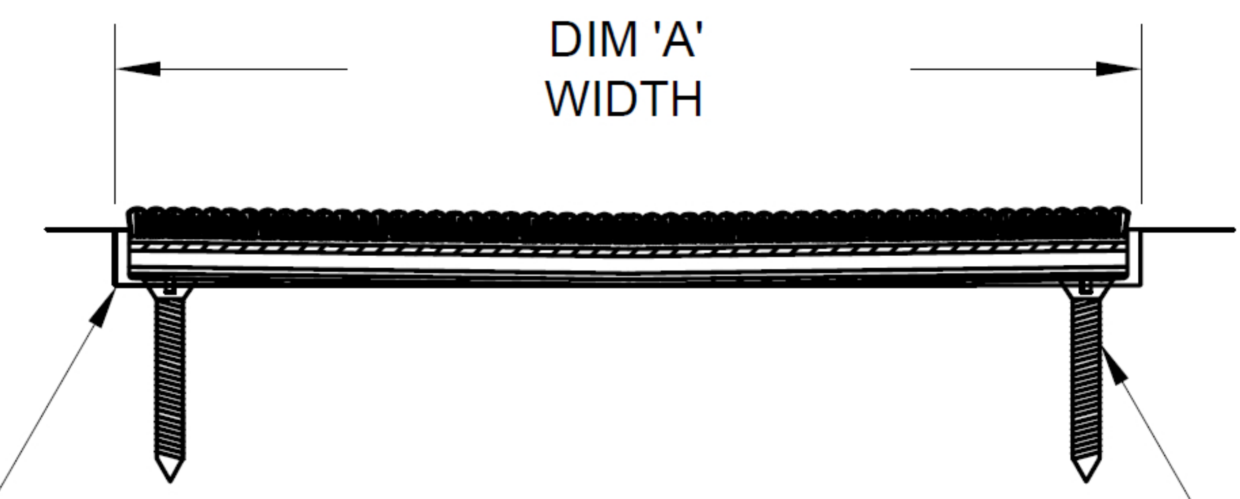
SECTION X-X
