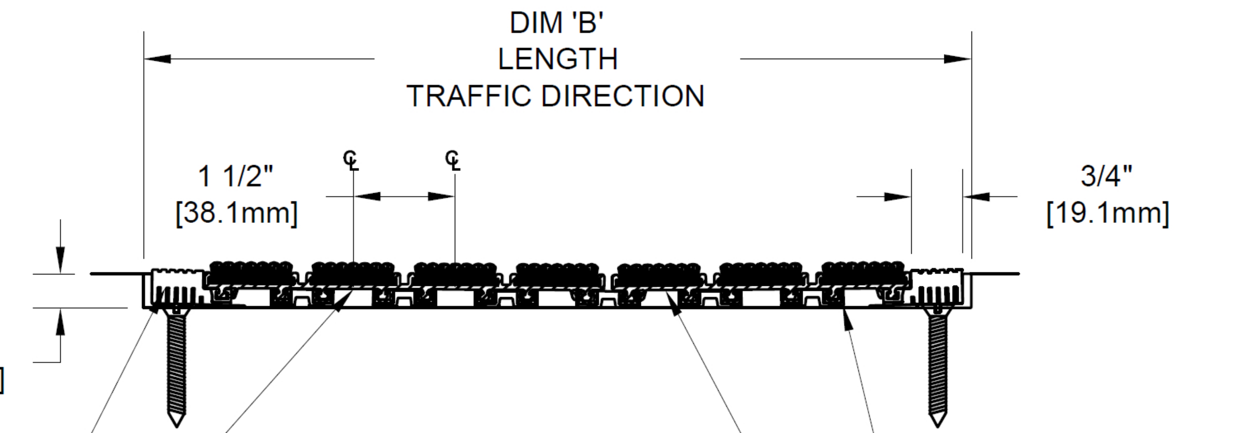
SECTION Y-Y
